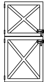
8034 ALL STEEL TOP & BOTTOM DOORS W/CROSSBUCKS
