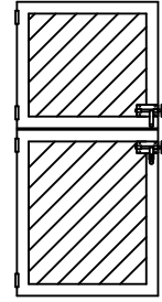
8018 WOOD INFILL IN TOP & BOTTOM DOORS
