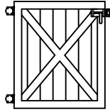
7414-H STRAIGHT TOP VERTICAL WOOD W/CROSSBUCKS
