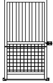
7030-S TOP BARS 2" SQ MESH KICK STRIP
