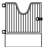
7510-H YOKE TOP W/ CLOSE BAR 2" O.C.
