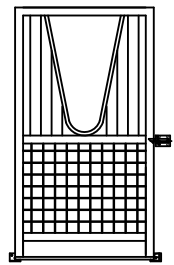
7130-S YOKE / BARS 2" SQ MESH KICK STRIP
